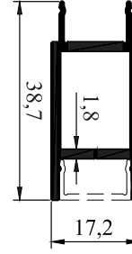
1700-214 YAN KASA 0.470 KG/M
