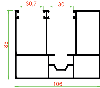
TG-104 YAN KASA (ÜST) 2.190 KG/M
