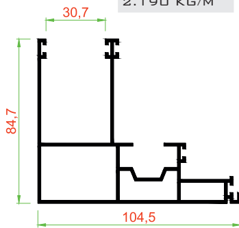
TG-103 YAN KASA (ALT) 1.169 KG/M
