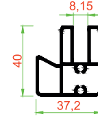
TGT-106 KENET (TEK CAM) 0.913 KG/M
